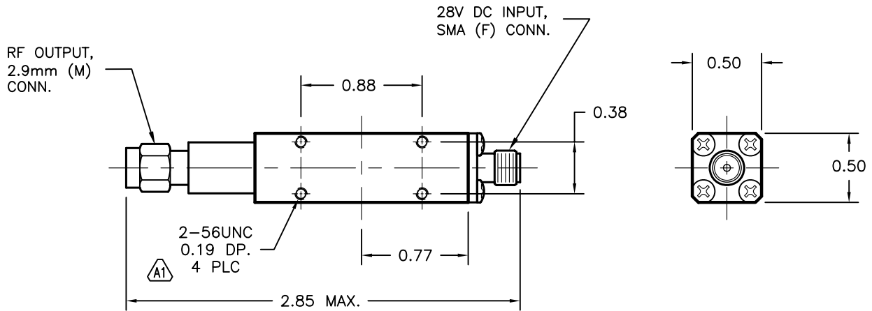
"V" TYPE (32dB OUTPUT)
