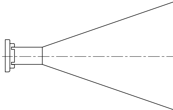
WR62 STD COVER FLANGE (UG 1665/U)
