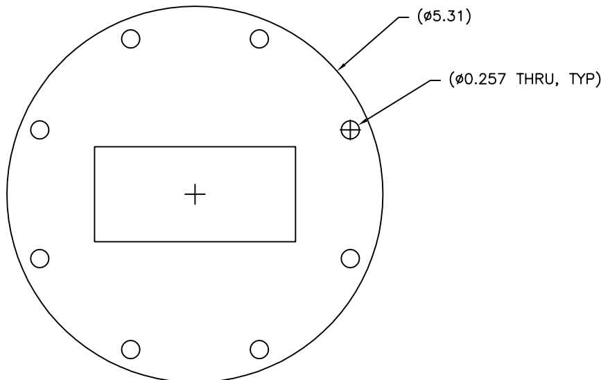
WR284 STD COVER FLANGE (UG-584/U)
