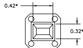
*INSIDE DIMENSION
